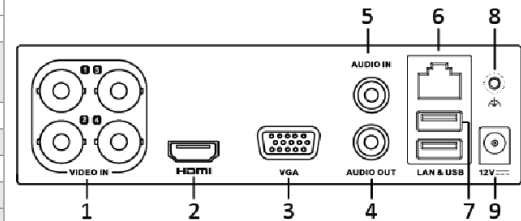
Rear Panel of HSVR-04MT
