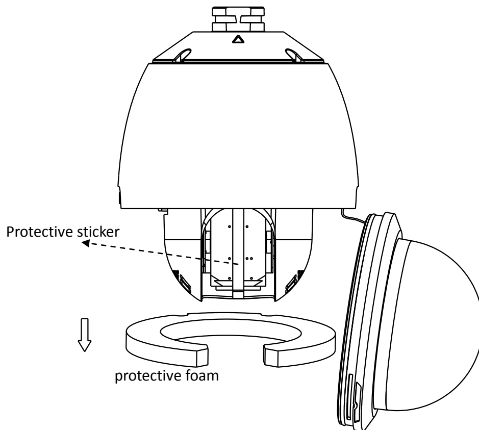
Figure 1-2 Disassemble the Speed Dome
