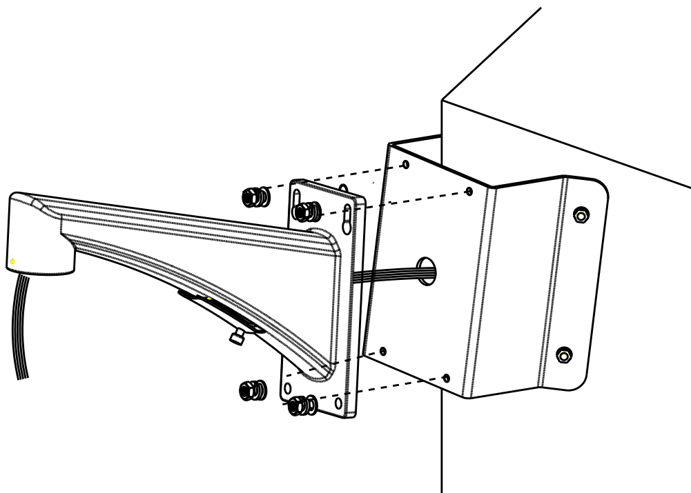
Figure 2-9 Secure the Wall Mount to the Corner
