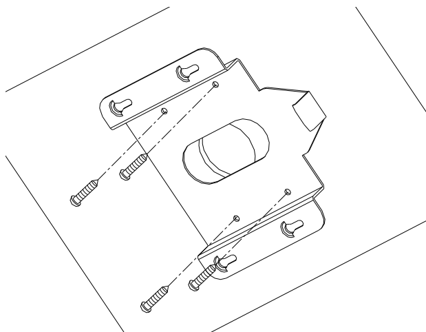
Figure 2-24 Secure the Mounting Base
