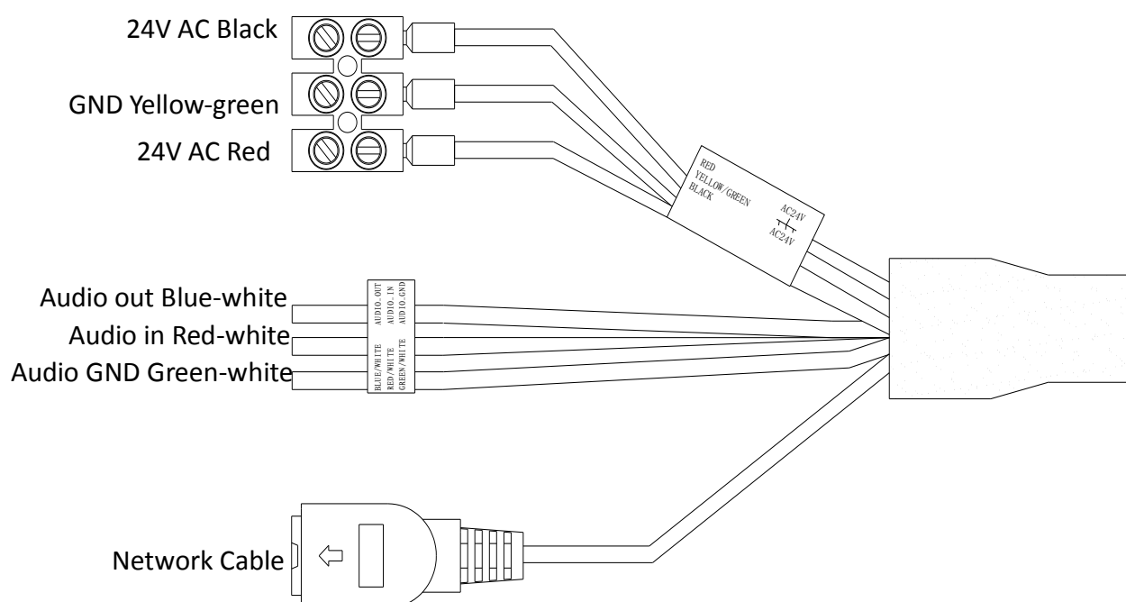
Figure 1-10 Cables of Network Speed Dome
