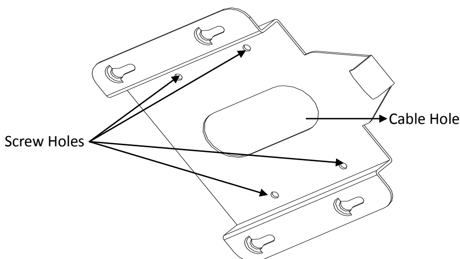
Figure 2-23 Mark the Screw Positions
