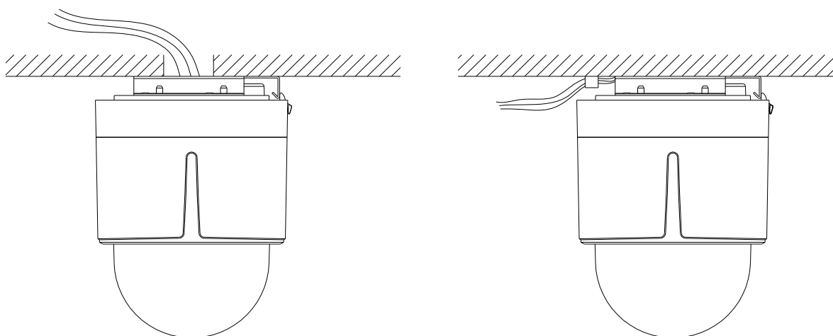
Figure 2-22 Cabling for Ceiling Mounting
