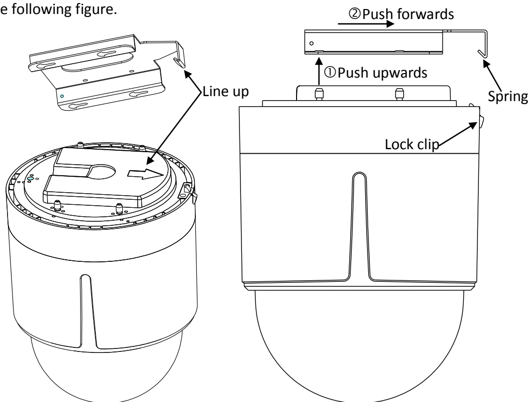
Figure 2-25 Attach the Back Box to the Mounting Base
