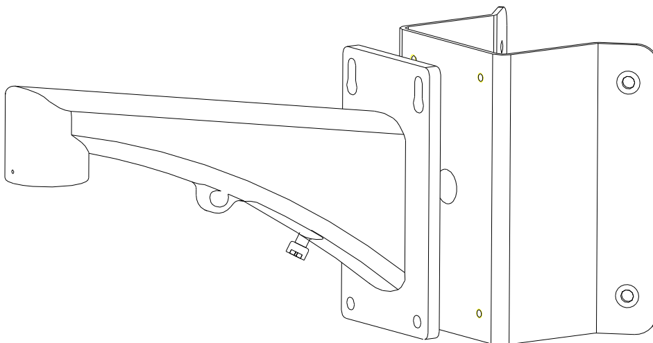
Figure 2-5 Wall Mount
