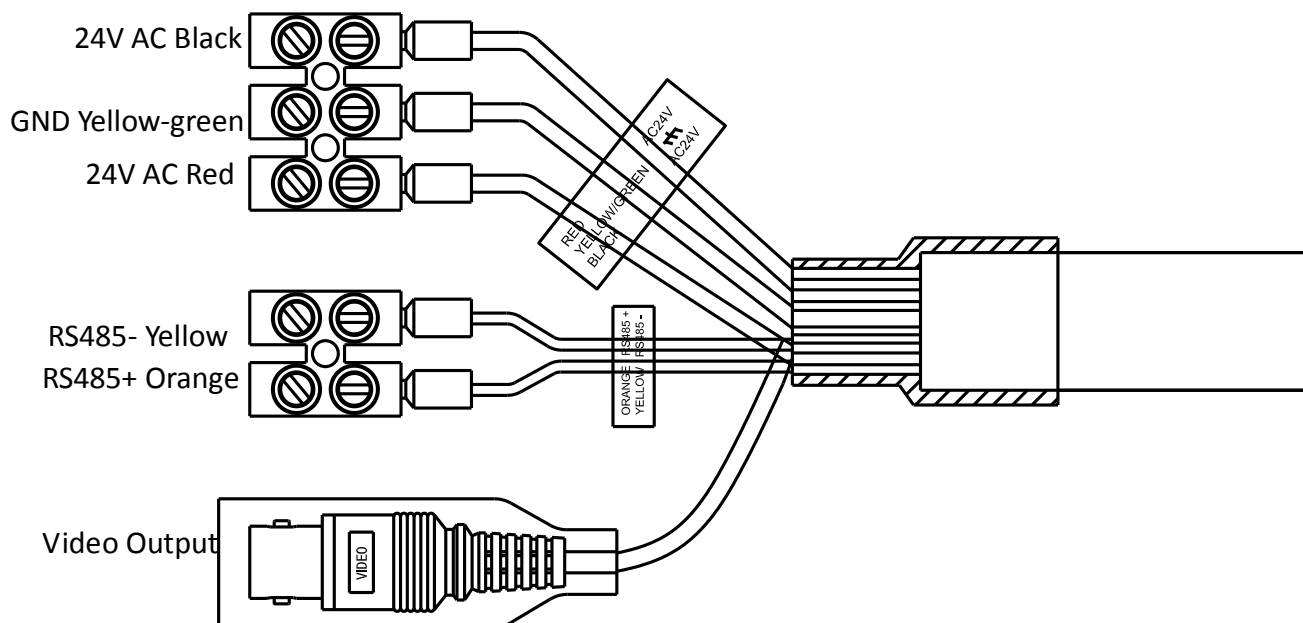
Figure 1-9 Cables of Analog Speed Dome
