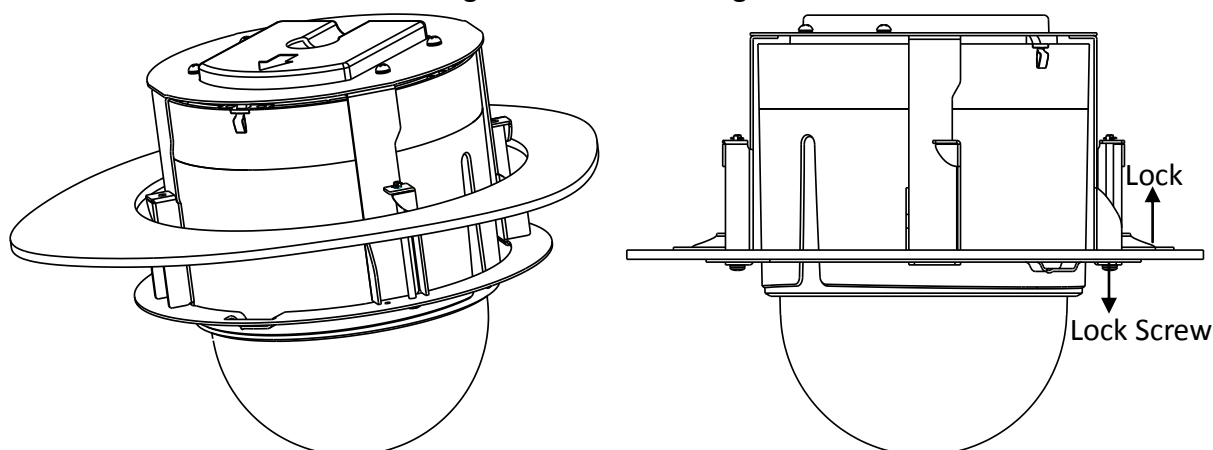
Figure 2-20 Install the back box
