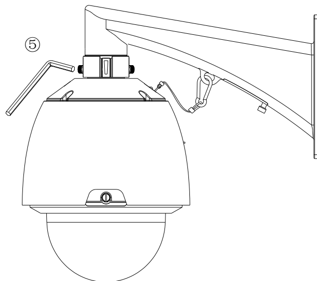
Figure 1-8 Tighten the Lock Screws
