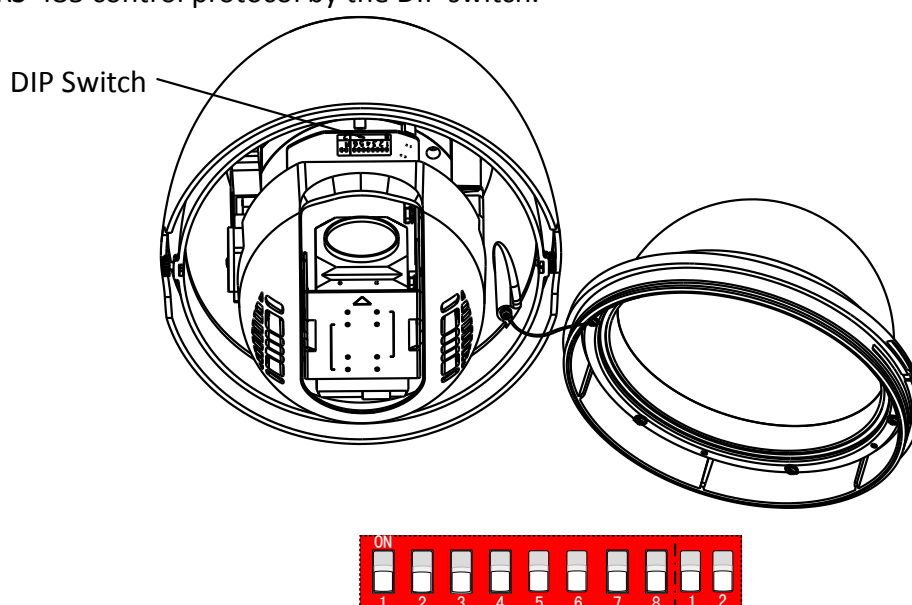
Figure 1-11 DIP Switch Settings
