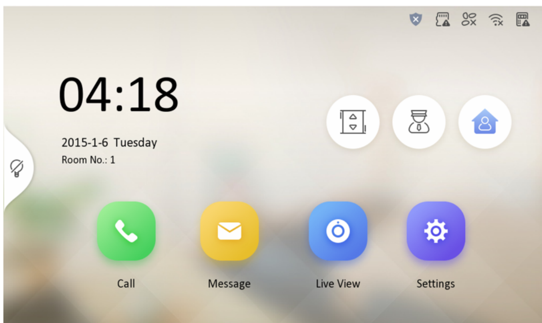
Figure 1-30 Main Page
