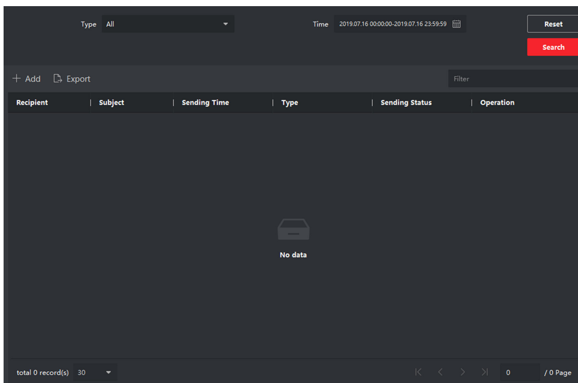
Figure 4-25 Search Notice
