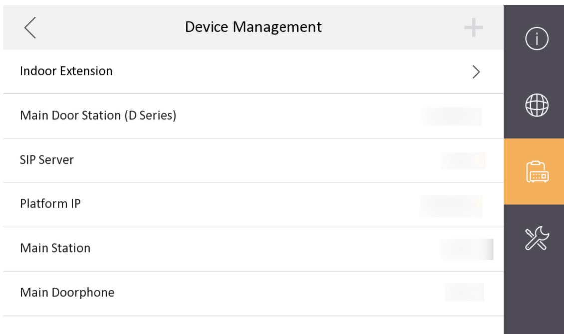
Figure 1-11 Device Information
