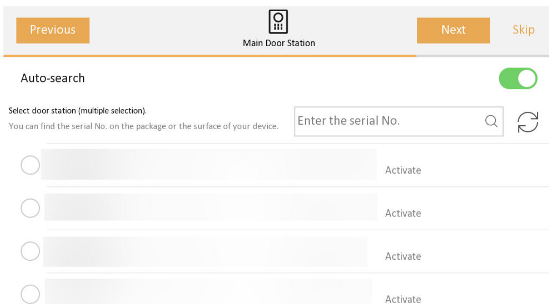
Figure 1-6 Related Device
