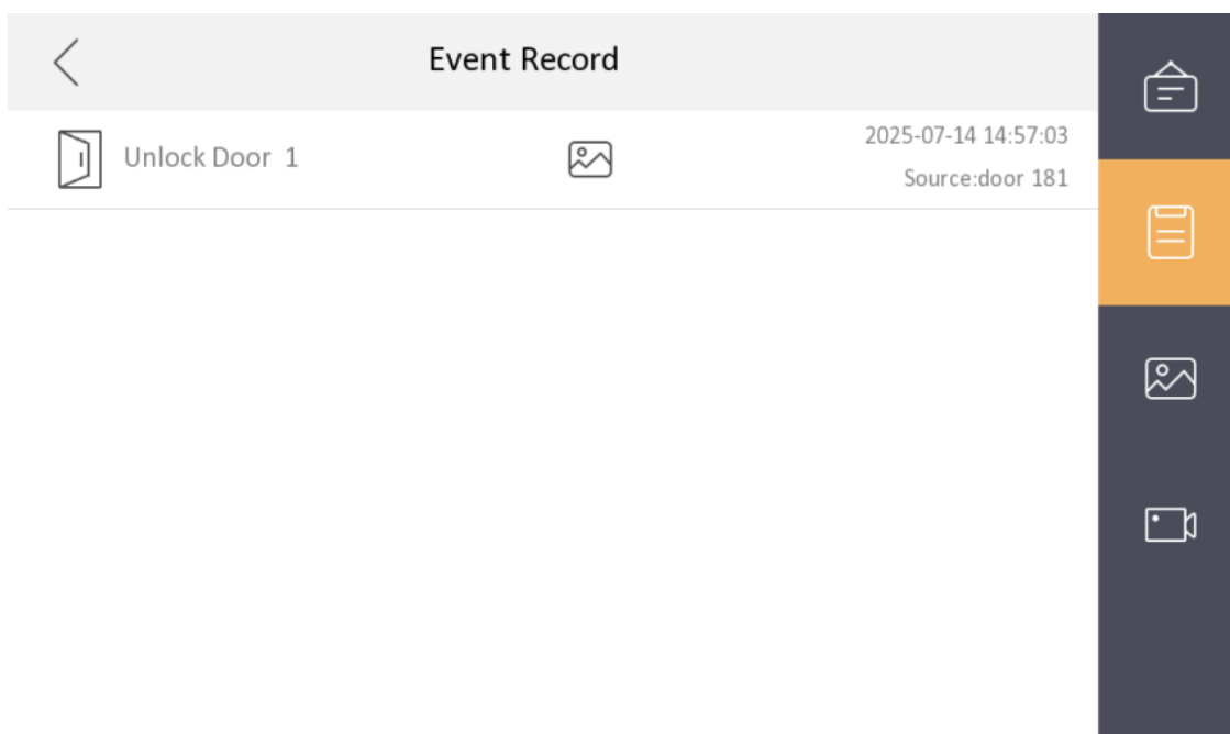
Figure 3-12 Event Record
