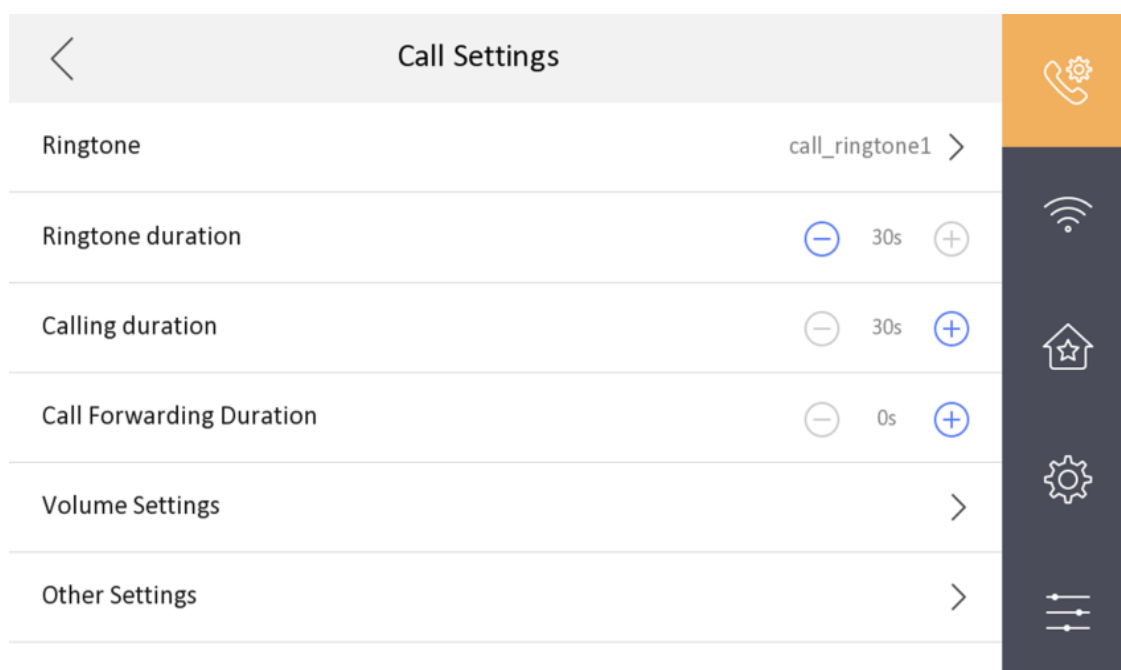
Figure 1-29 Call Settings
