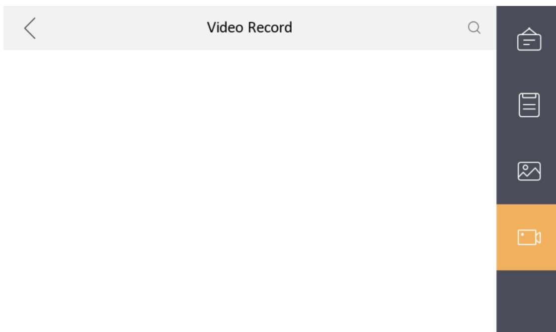
Figure 3-13 Video Record
