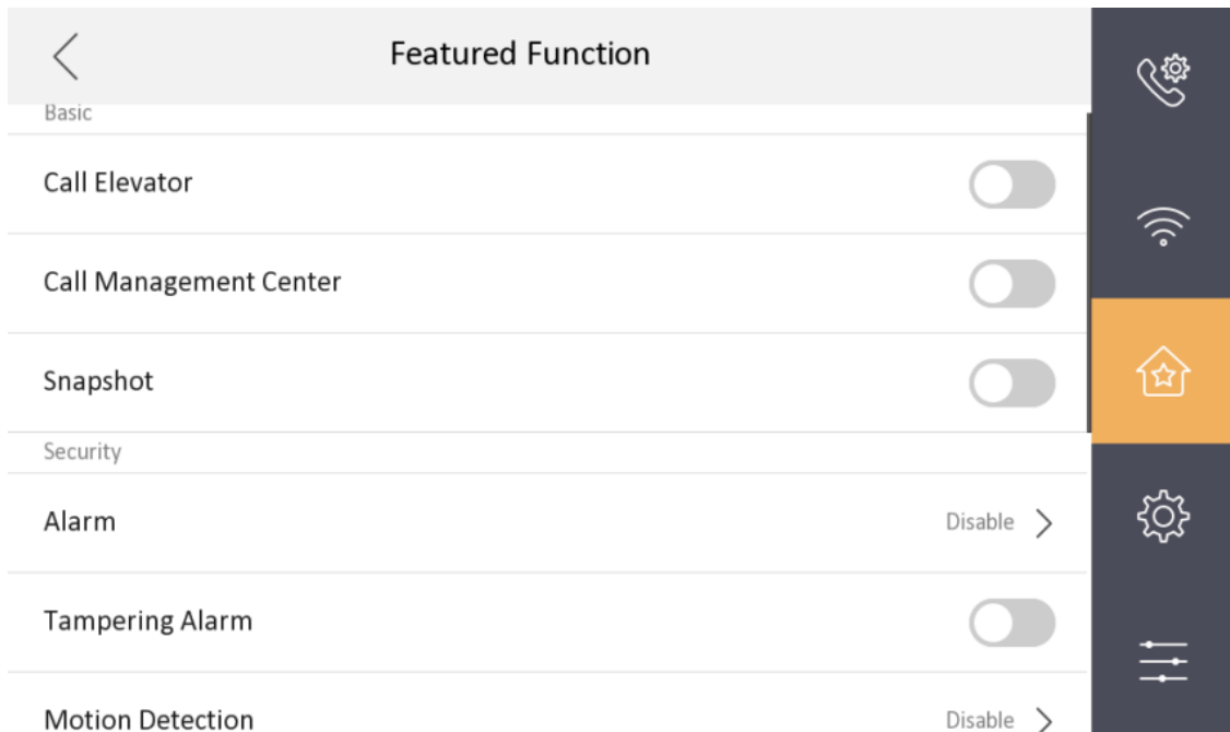
Figure 1-26 Featured Function
