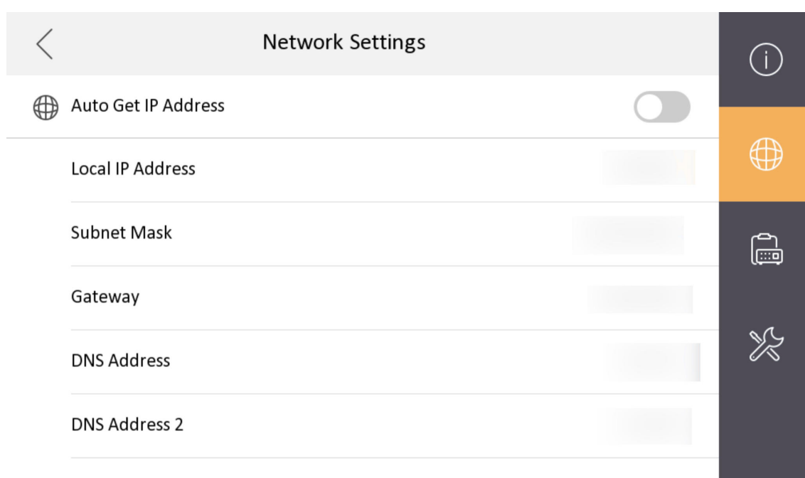
Figure 1-8 Network Information
