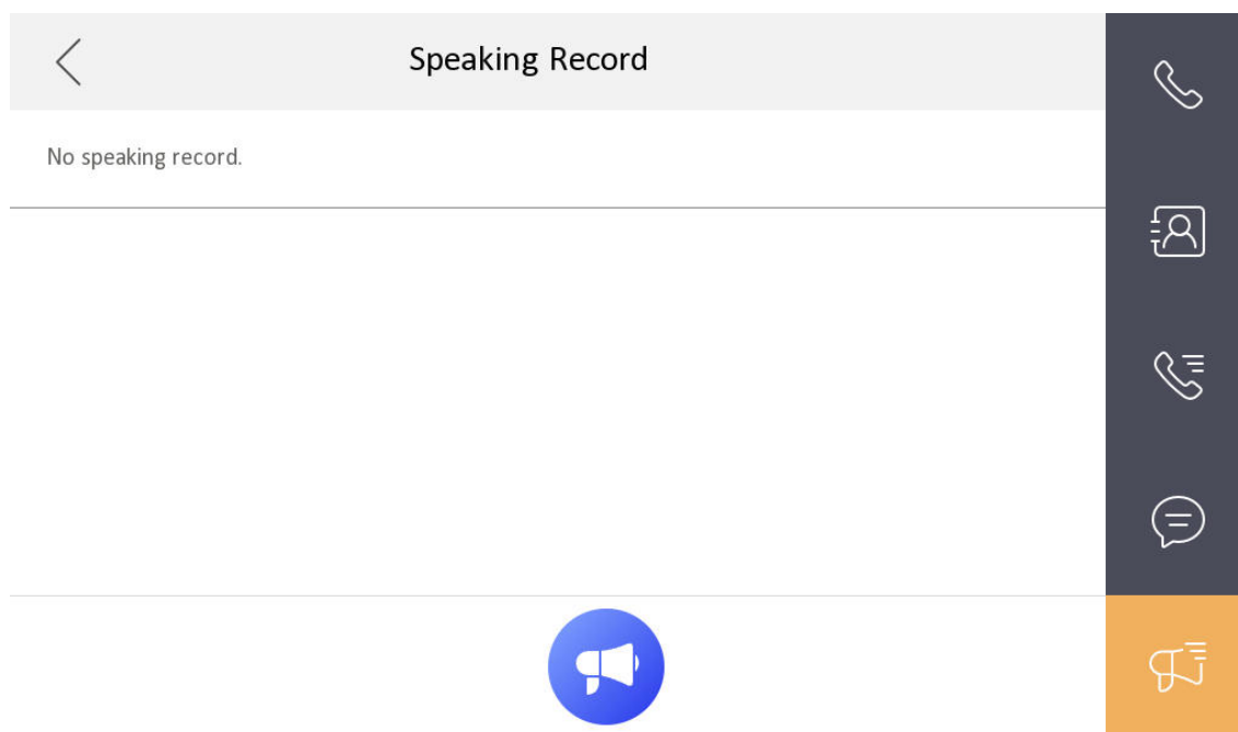
Figure 3-11 Speaking Record
