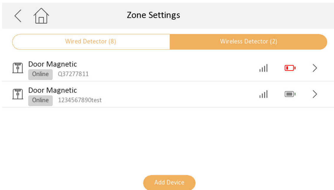
Figure 1-15 Zone Settings
