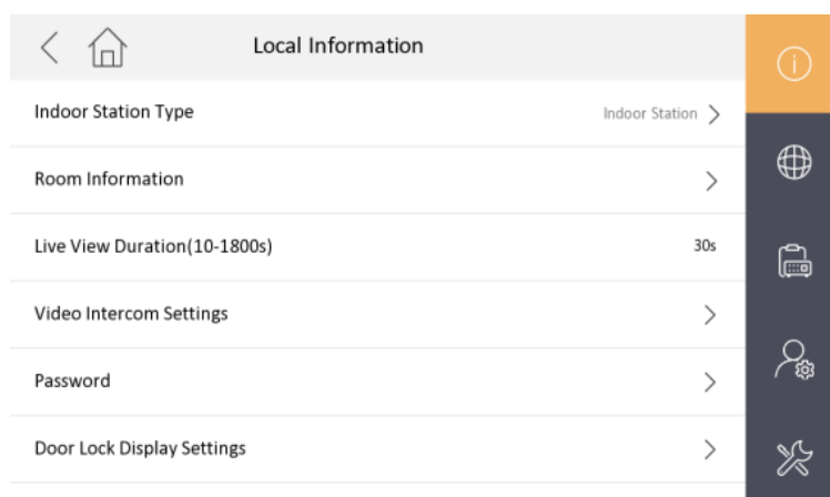
Figure 1-22 Local Information
