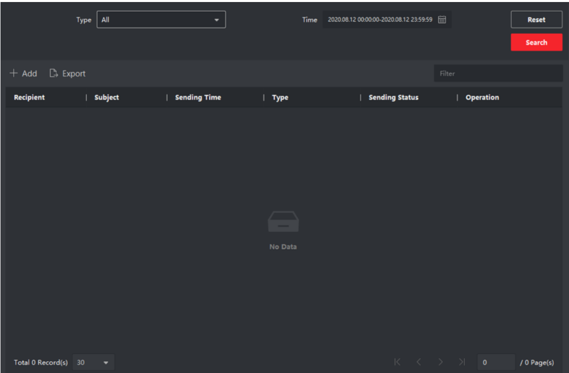
Figure 4-22 Release Notice
