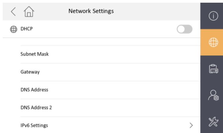
Figure 1-12 Network Settings-IPv6
