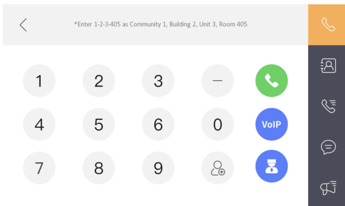
Figure 3-10 Call Resident
