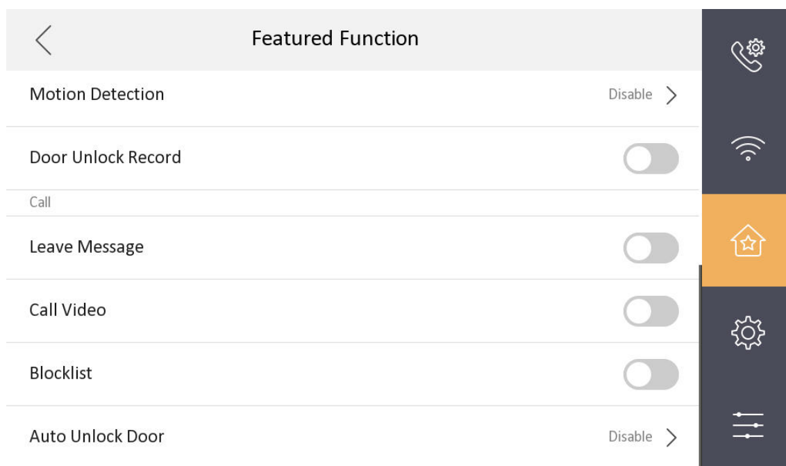
Figure 3-1 Leave Message
