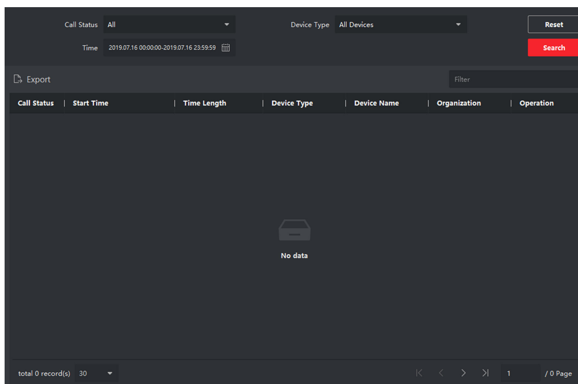
Figure 4-21 Call Log
