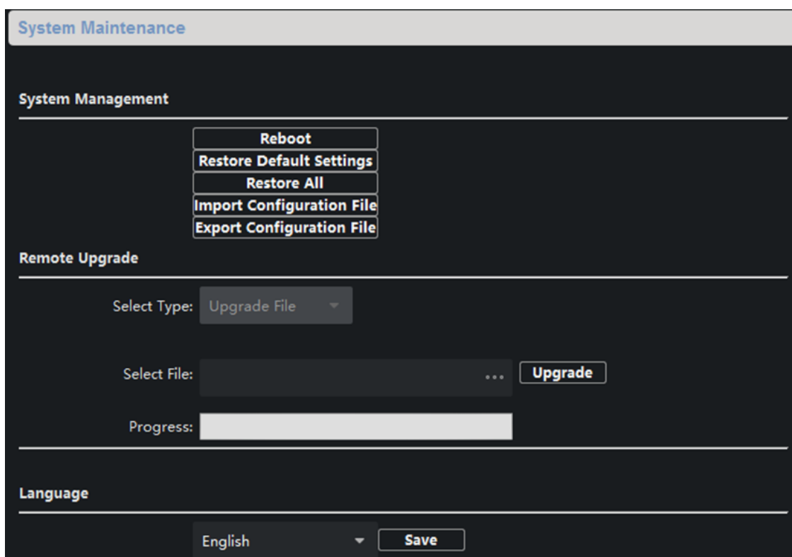
Figure 4-5 System Maintenance
