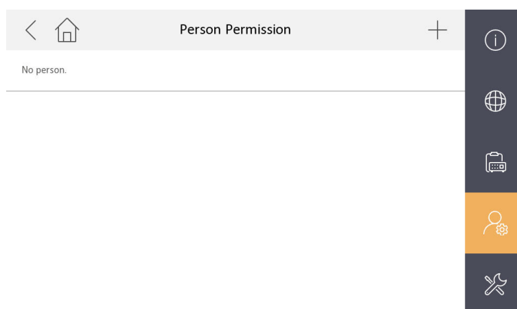
Figure 1-32 Person Permssion
