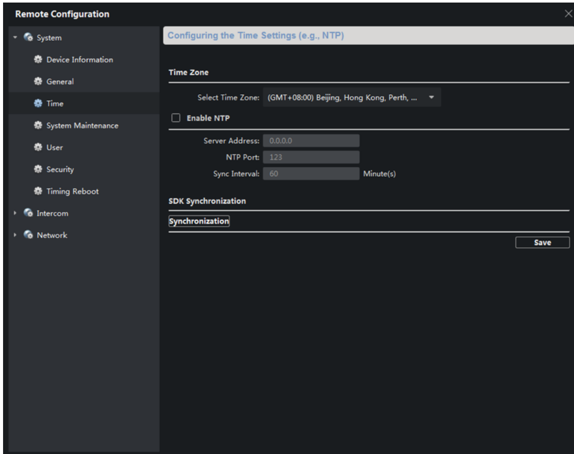
Figure 5-4 Synchronize Time
