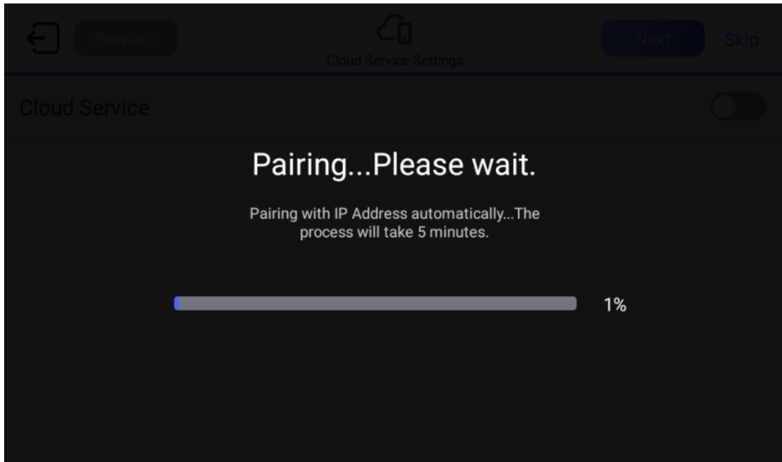
Figure 3-8 Pairing
