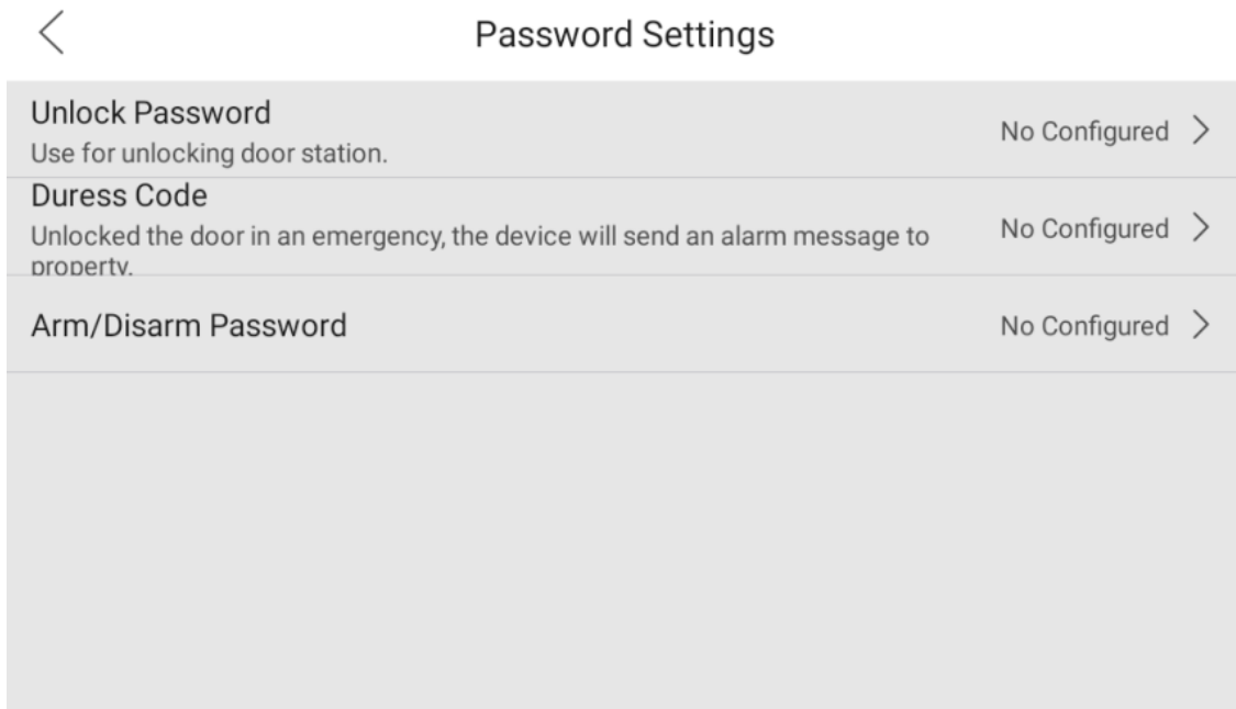
Figure 3-23 Password Settings
