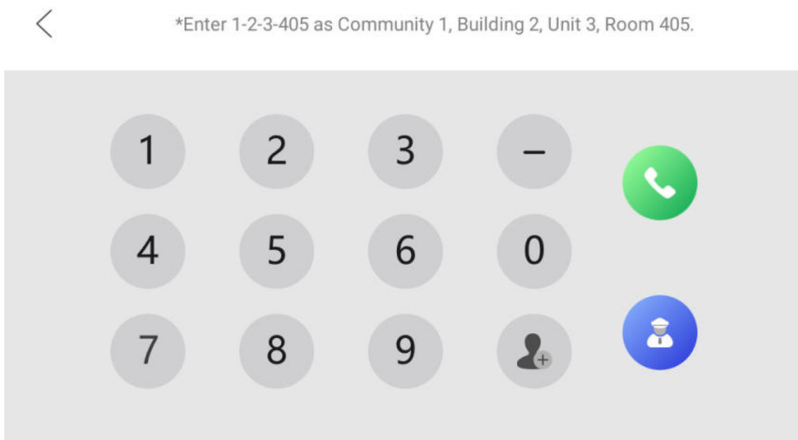
Figure 4-4 Call Resident
