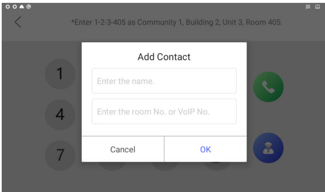
Figure 4-3 Add Contact
