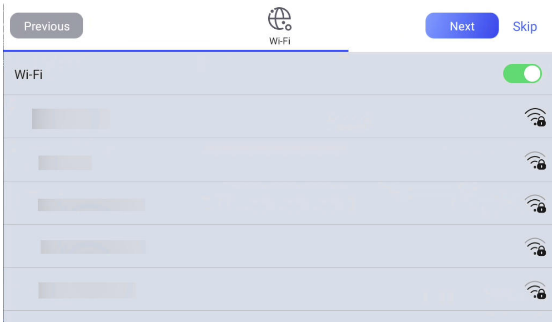
Figure 3-5 Wi-Fi
