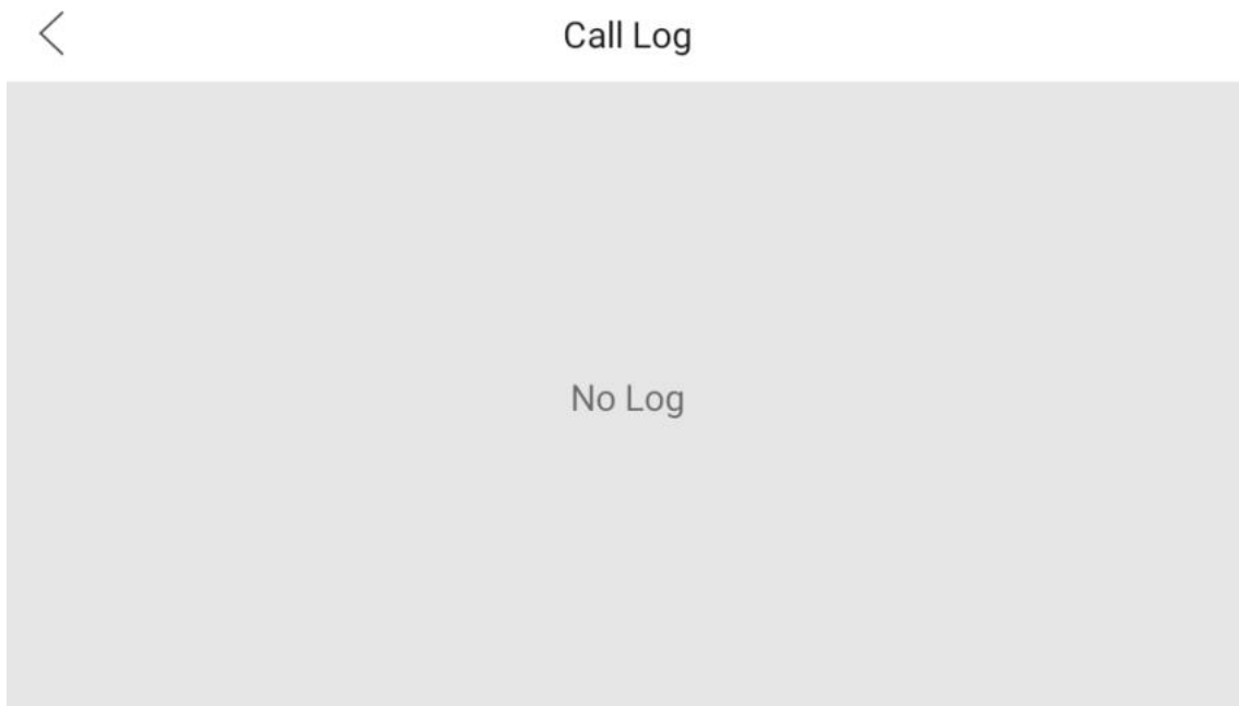
Figure 4-5 Call Logs
