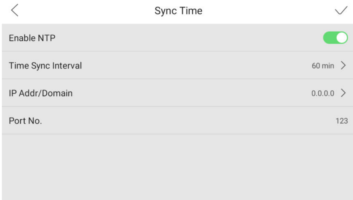
Figure 3-31 Sync Time
