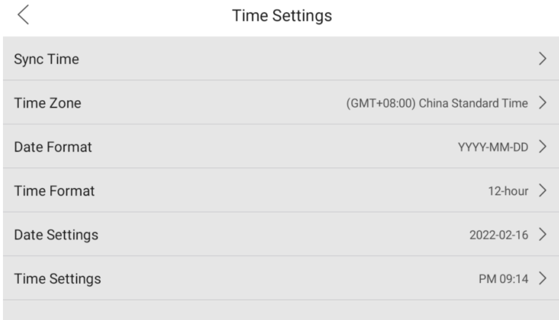
Figure 3-30 Time Settings
