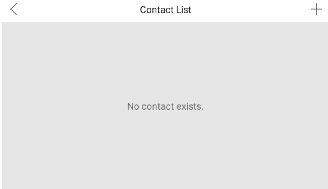
Figure 4-2 Contact List
