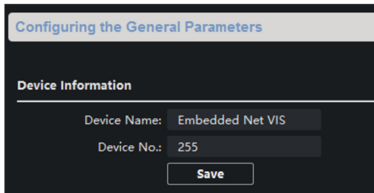
Figure 5-3 General
