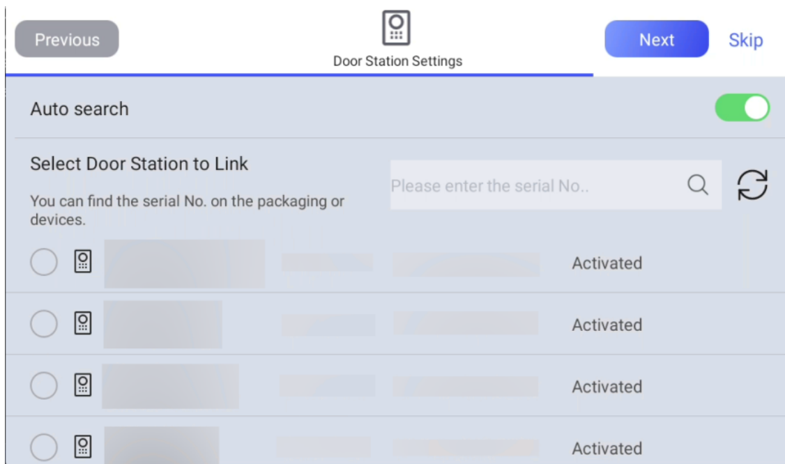
Figure 3-6 Related Device
