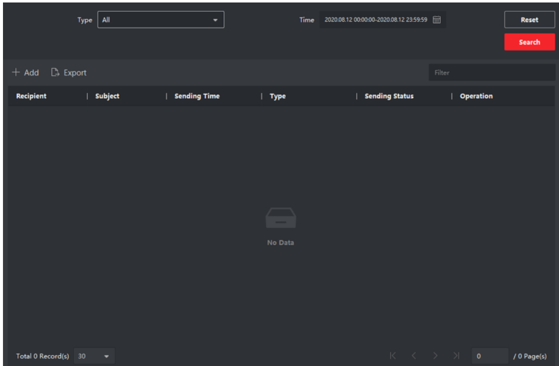
Figure 5-21 Release Notice
