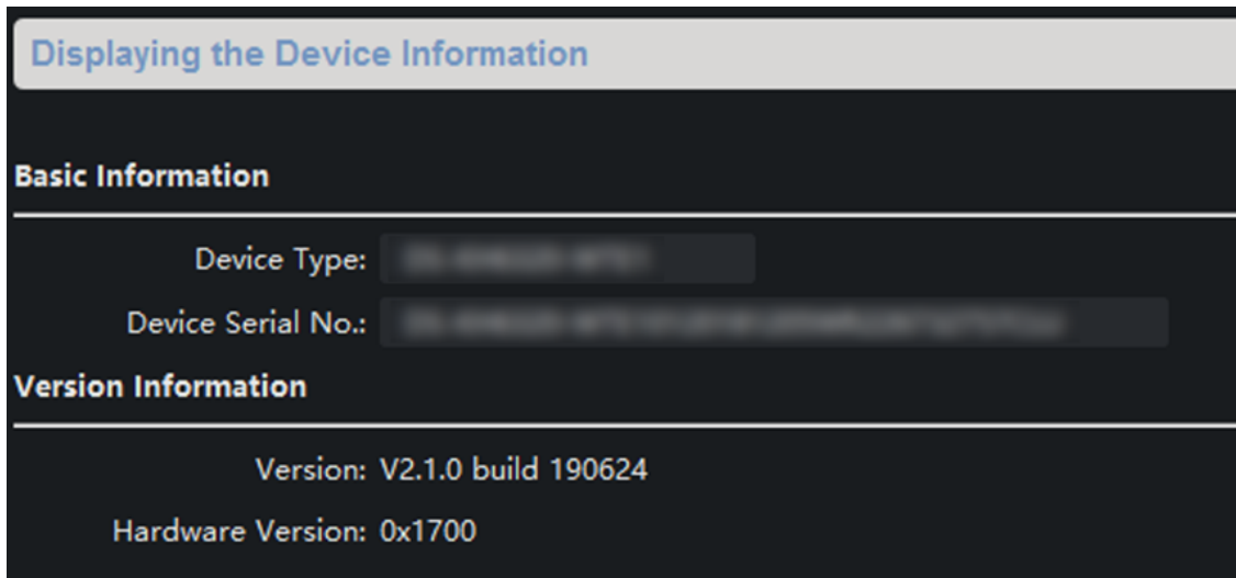
Figure 5-2 Device Information
