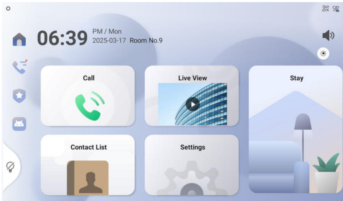
Figure 2-1 Main Page
