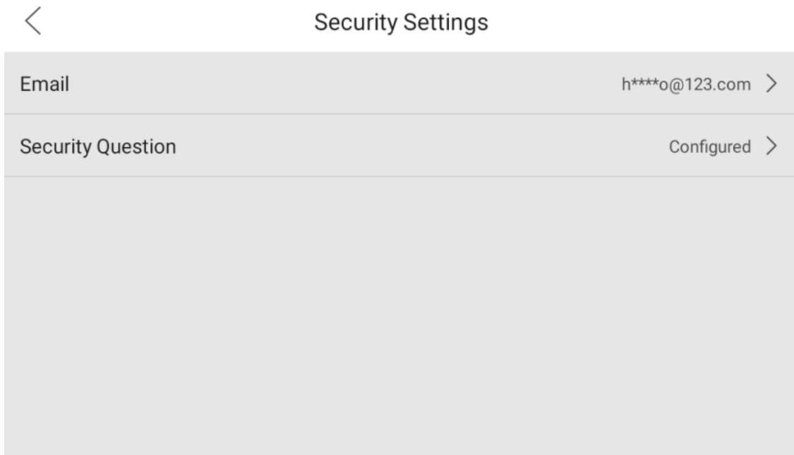
Figure 3-22 Security Settings
