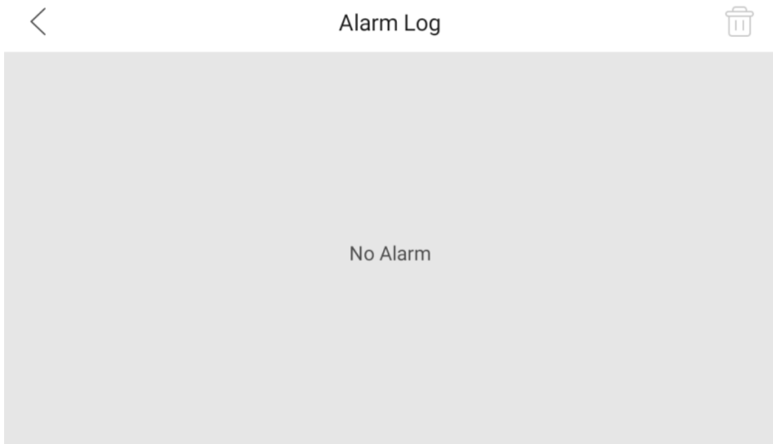
Figure 4-10 Alarm Logs
