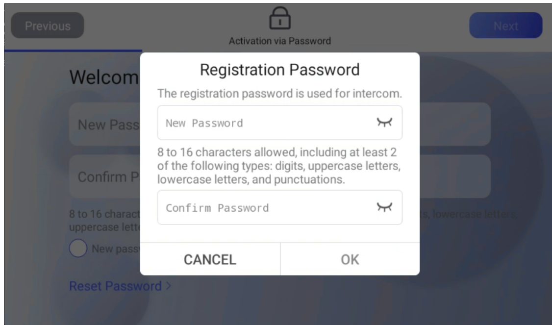
Figure 3-3 Registration Password
