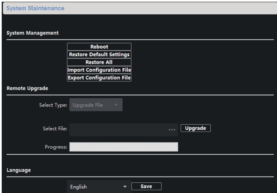
Figure 5-5 System Maintenance
