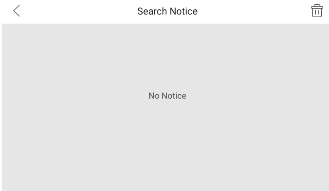
Figure 4-9 Search Notice
