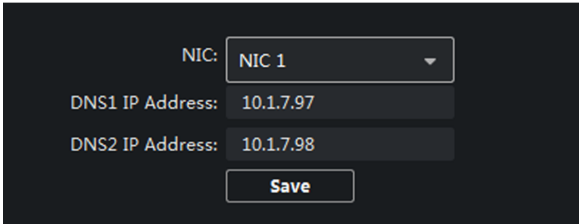
Figure 5-16 DNS Settings
