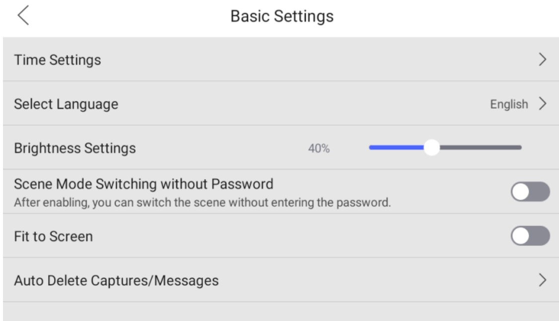
Figure 4-12 Basic Settings
