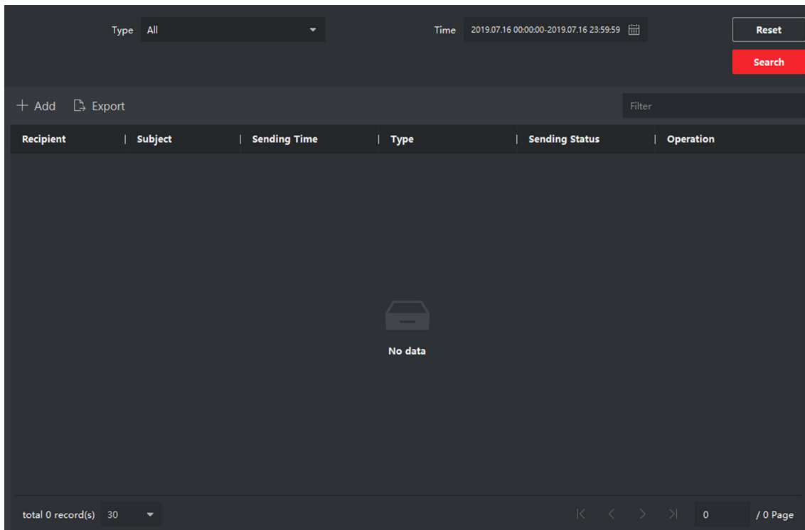
Figure 5-24 Search Notice
