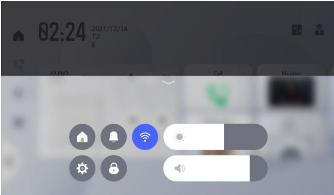
Figure 2-5 Control Center
