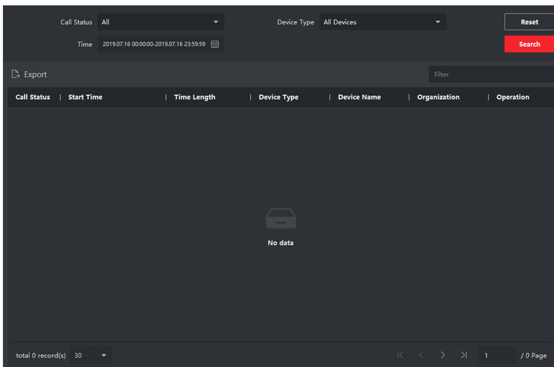
Figure 5-20 Call Log
