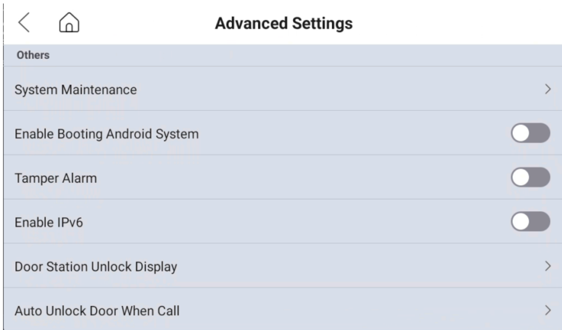
Figure 3-18 Advanced Settings
