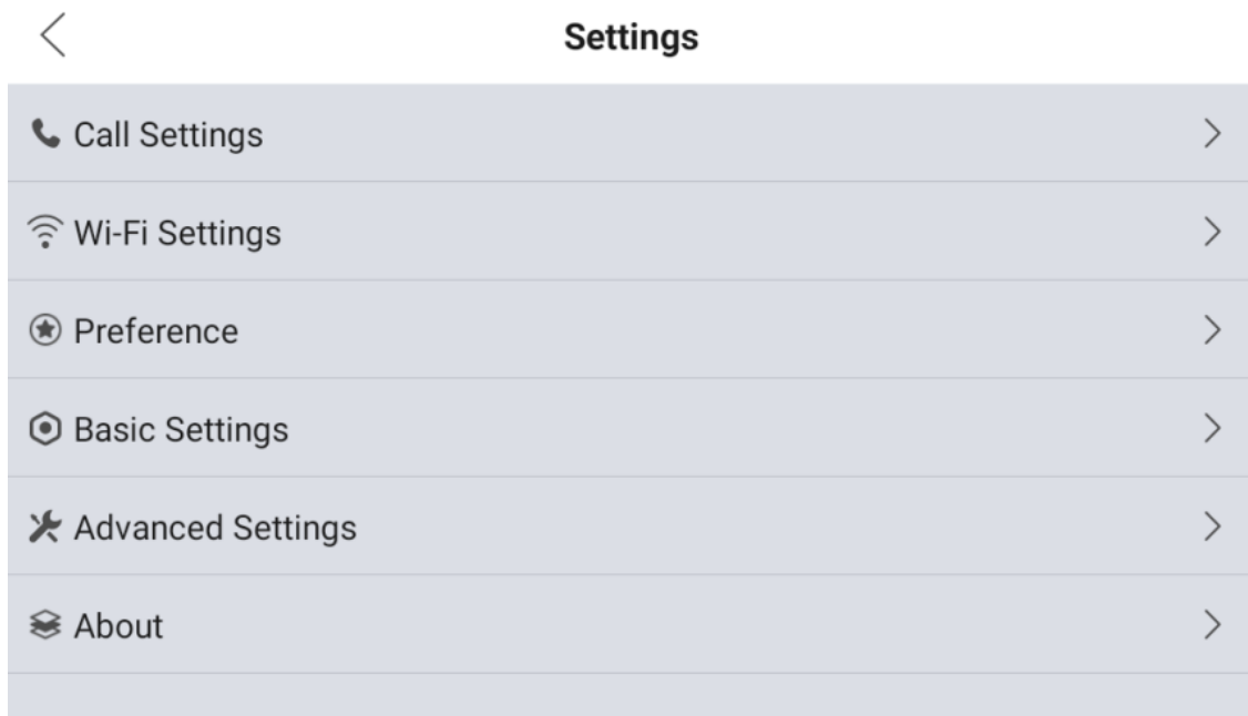
Figure 3-9 Settings
