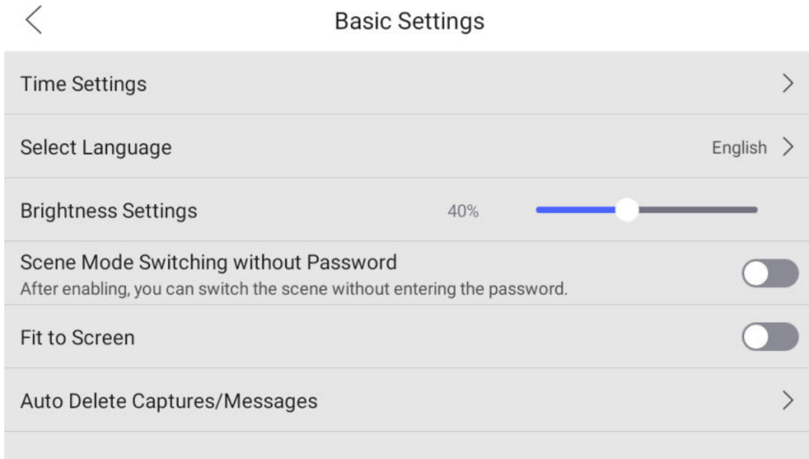
Figure 3-27 Basic Settings
