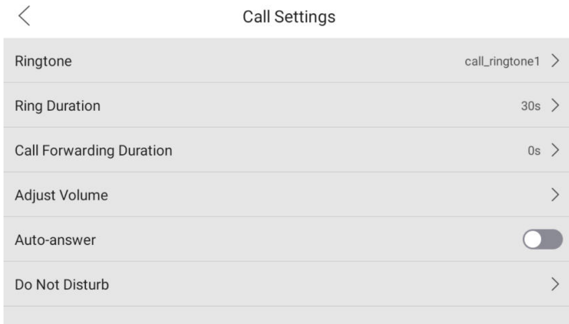
Figure 3-32 Call Settings
