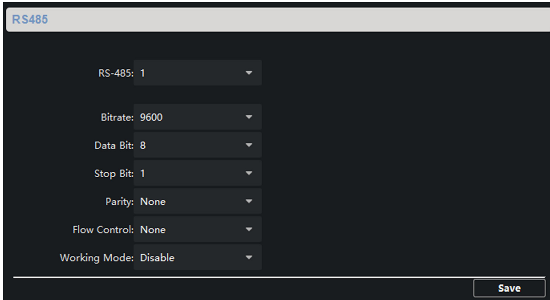
Figure 5-7 RS-485 Settings
