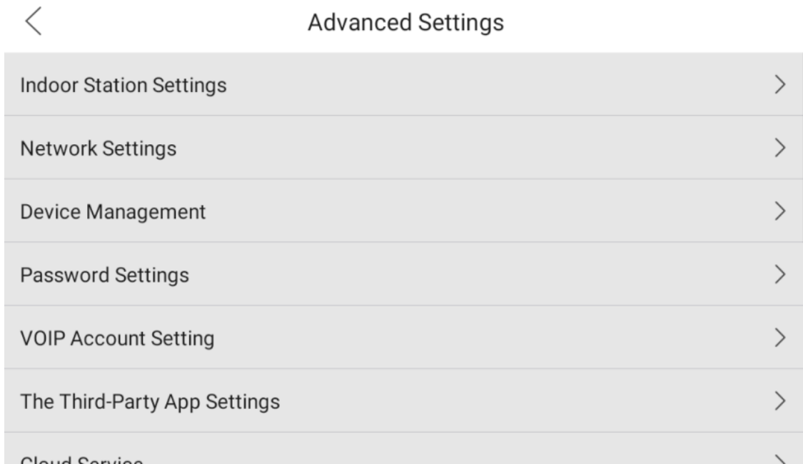
Figure 3-29 Advanced Settings
