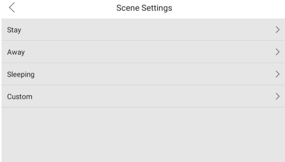
Figure 4-7 Scene Settings
