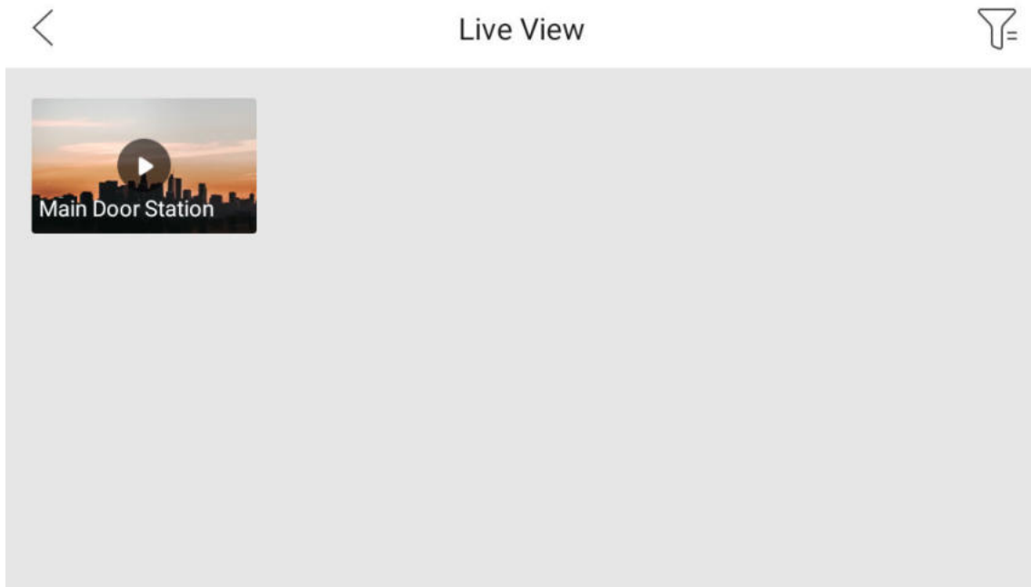
Figure 4-6 Live View
