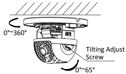
Figure 2-5 Angle Adjustment
