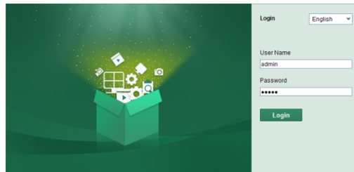
Figure 4-1 Login Interface
