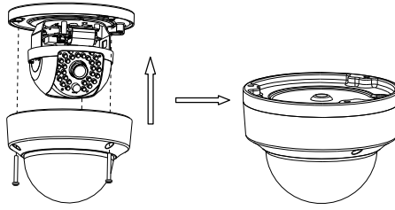
Figure 2-6 Bubble Reinstallation
