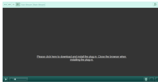
Figure 4-2 Download Plug-in
