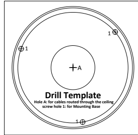
Figure 2-1 Drilling Template
