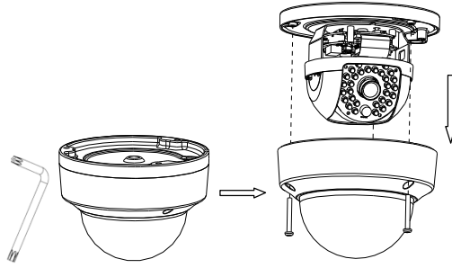
Figure 2-2 Remove the Bubble
