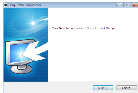
Figure 4-3 Install Plug-in (1)
