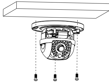
Figure 2-3 Fix the Mounting Base
