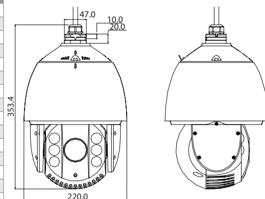
DIMENSIONS (mm)
