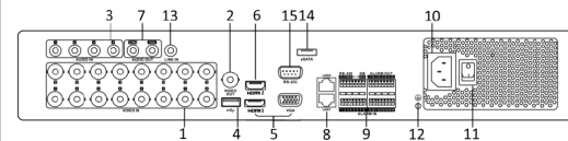
Rear Panel of HAVR-16HT4
