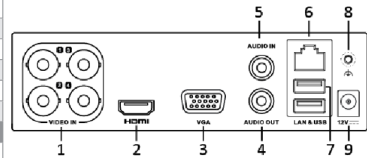
Rear Panel of HAVR/04MT
