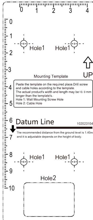
Figure 3-2 Mounting Template
