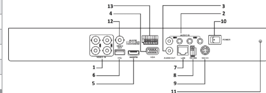
Rear Panel of HAVR-04HT
